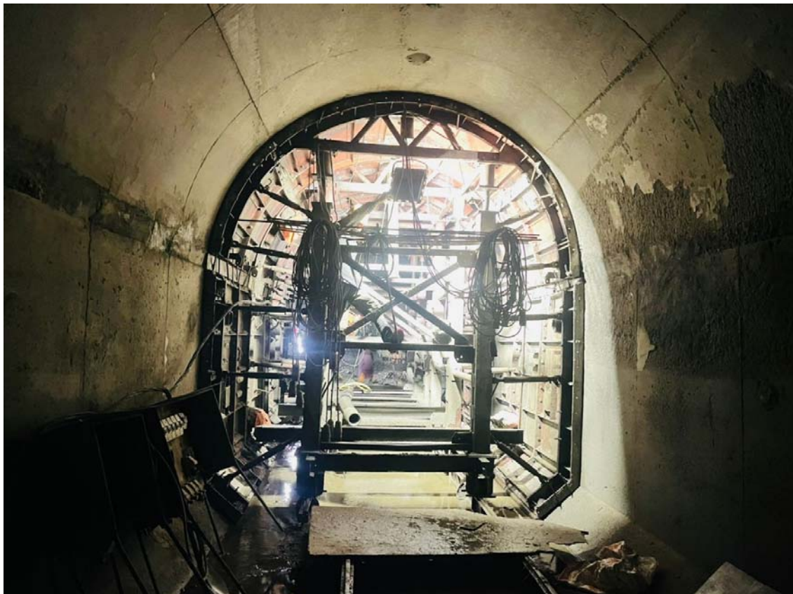
Gantry Preparation for the lining work in Face 1
