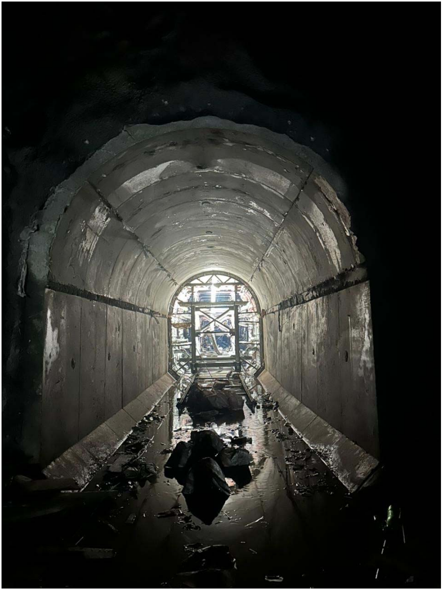
Face 4 full lining work
